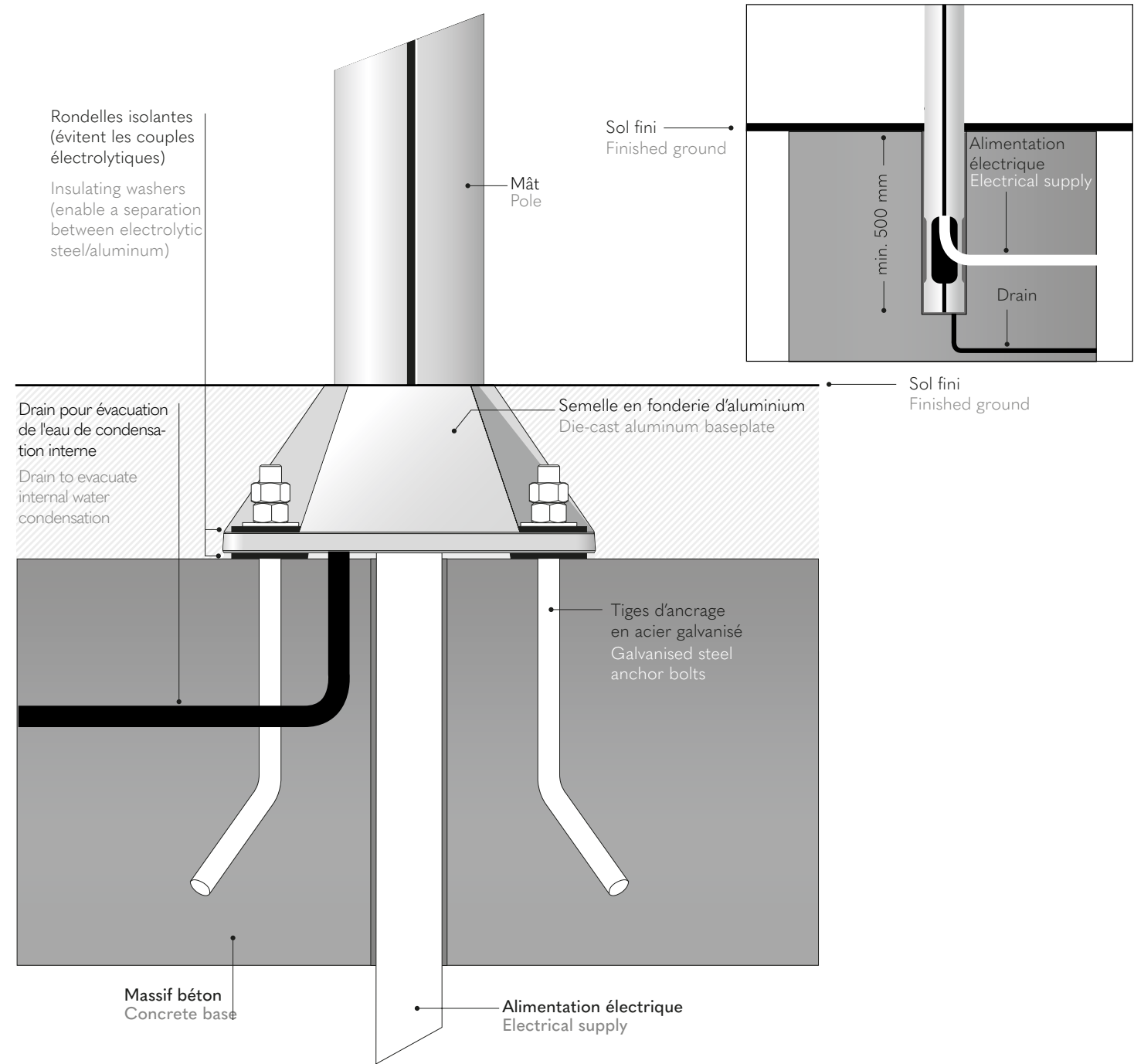
Configuration type d’une base de mât Typical configuration of a pole base
